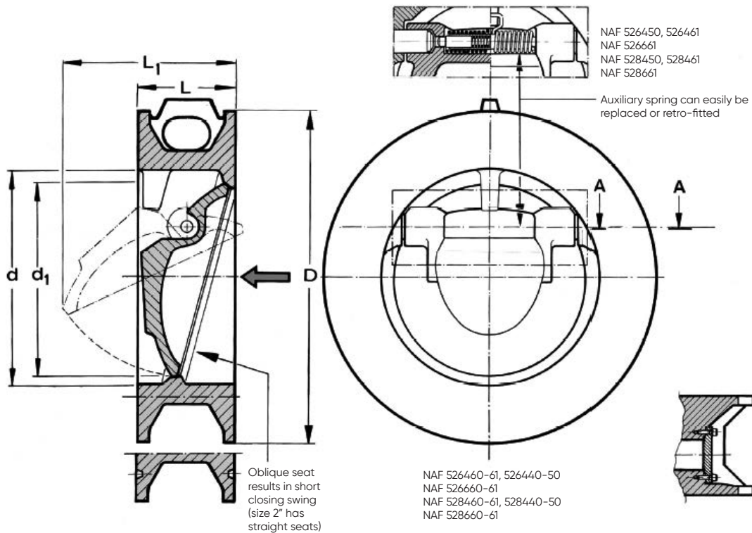
DIMENSIONS (TABLE 6)
