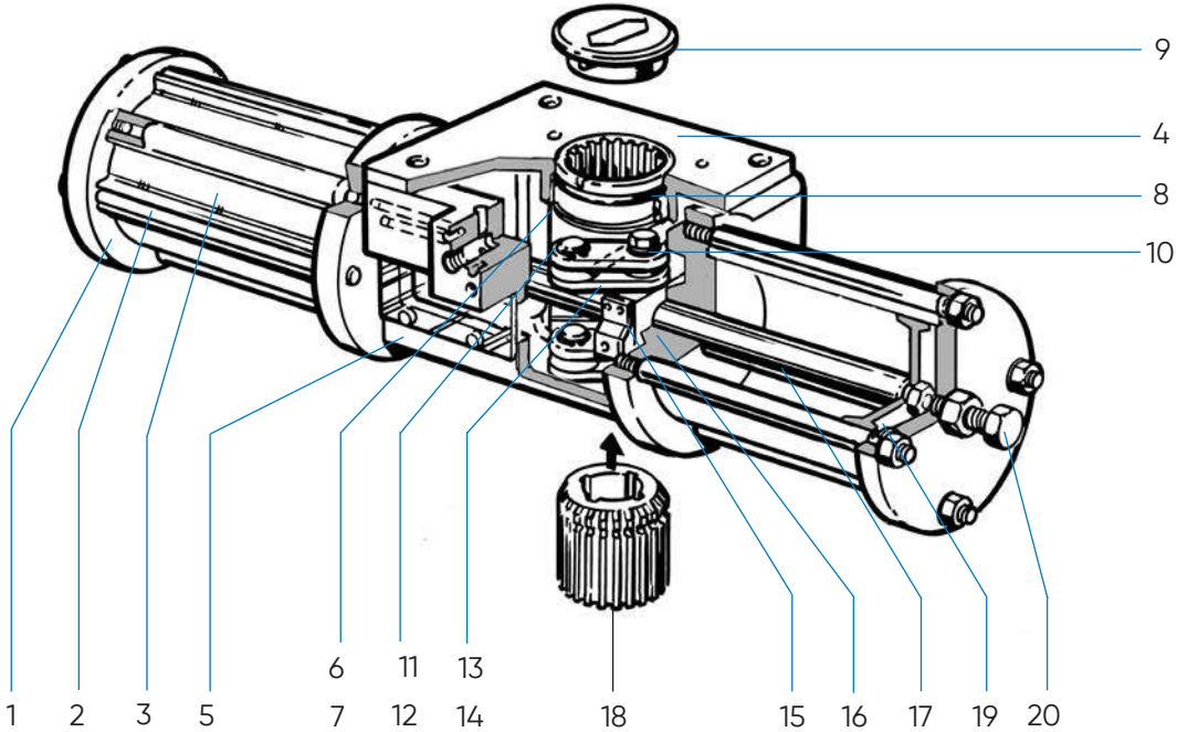
791.92/94 SIZE 0 -3 WITH SPRING RETURN
