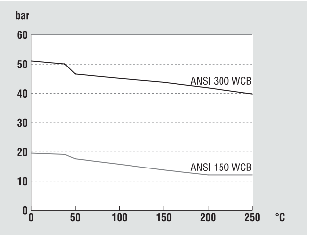
Carbon steel body (WCB)
