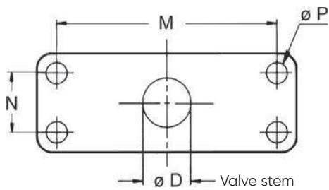
NAF standard for actuator mounting
