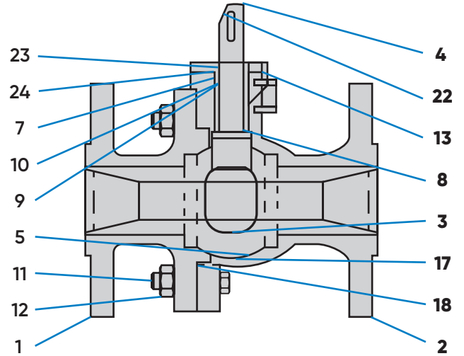
MAX WORKING PRESSURE PN VALVE
